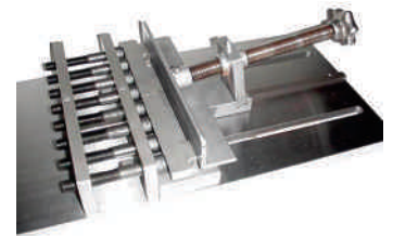
Bolt Cutoff Jig
